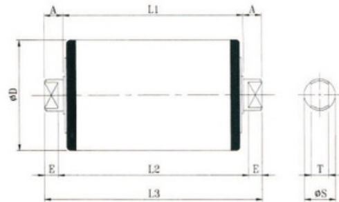
Flat Carrier Roller
