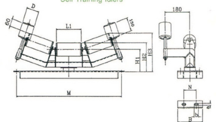
Self Training Idlers
