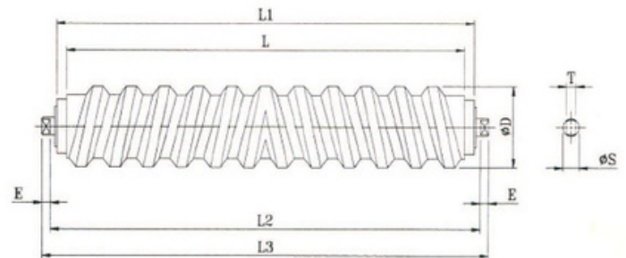
Spiral Return Roller
