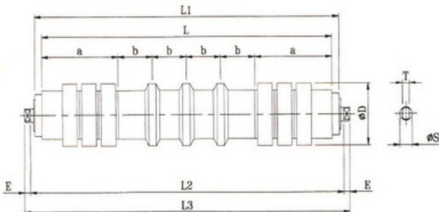
Rubber disc Return Roller
