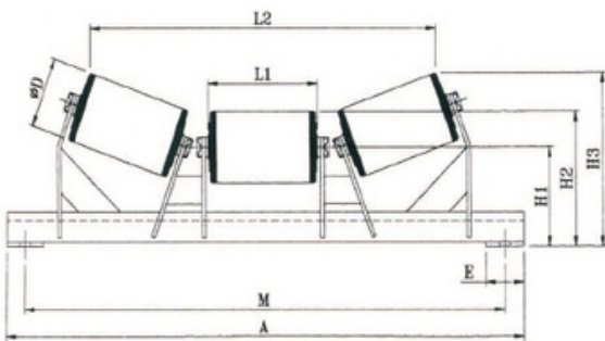
Trough Angle For Carrier Roller-Equal Rolls
